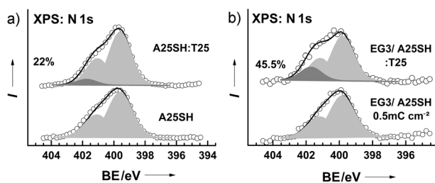
Figure 3. N 1s PE spectra of the reference A25SH monolayer (bottom, a) and mixed EG3/A25SH film fabricated by IPER with a dose of 0.5 \text{ mC cm}^{-2} (bottom, b) along with the spectra of the same films after the hybridization with T25 (top, a,b). The spectra are decomposed into individual contributions, which are shaded light gray for adenine and dark gray for thymine. The decomposition procedure was performed self-consistently and relied on well-known data for adenine- and thymine-based oligonucleotides. [5,30] Note that the spectra in the bottom traces were used as references for the decomposition of the spectra in the top traces.
